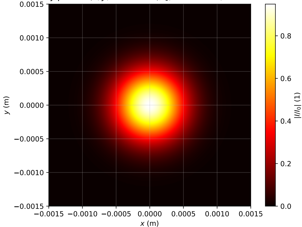
Intensity profile I(x, y, z = 0.557m)/I_0 , Pin=0.1Pcr, artificial time
